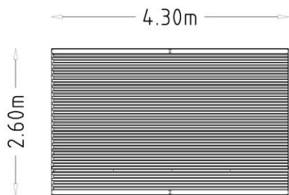
Bicycle Shelter Stella Vaulted Steel
